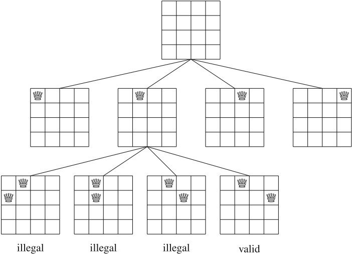
Fig. 2.3 Partial solutions to the queen problem using backtracking
