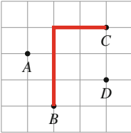
Manhattan distance
