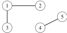
step 5: remove edge 2-4 number of components: 2
