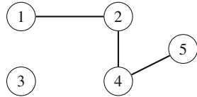
step 3: remove edge 2-5 number of components: 2
