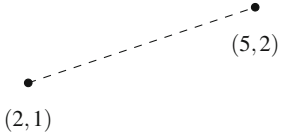
Euclidean distance
