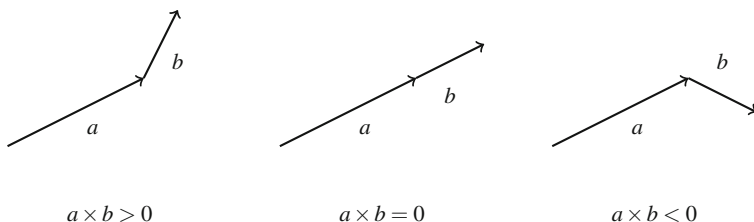
Fig. 13.2 Interpretation of cross products
